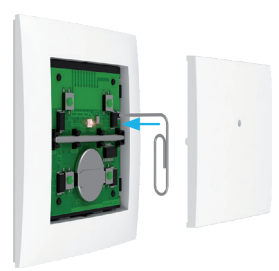
RFWB: By removing the controller flap, the pairing button is accessed.
