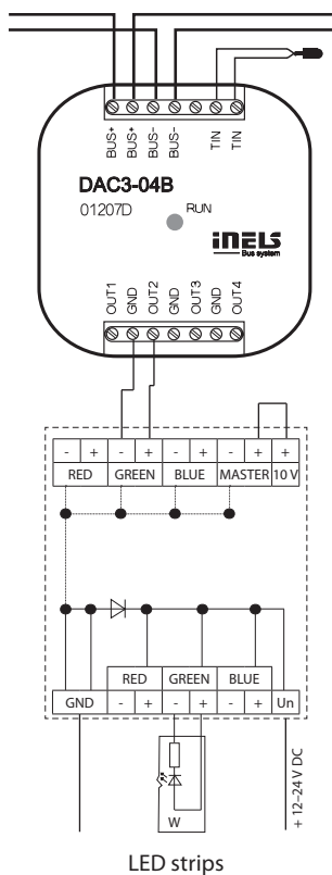
TERM 0(1)–10 V DC - monochrome LED strips
