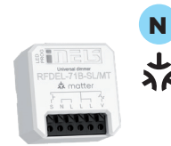
RFDEL-71B-SL/MT Universal dimmer, 1-channel – 1x 300 VA, MATTER
