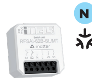
RFSAI-62B-SL/MT Switch unit with inputs for external buttons MATTER, 2x 8 A (total)
