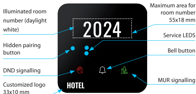
RFGS-230/SB (BLACK glass, ROUND)
