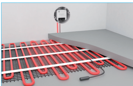
RFSTI-11B/SL Switch unit with external temperature sensor
