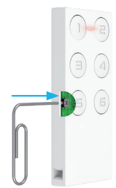
RF Key It is located on the side near the button number 5.
