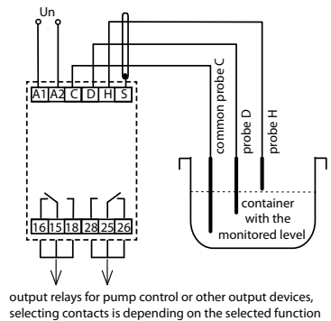
For controlling the level combination of upper and bottom probe
